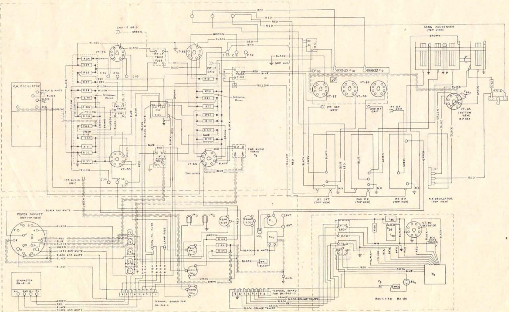
FIGURE 12. RADIO RECEIVERS BC-314-G AND BC-344-D, WIRING DIAGRAM.
