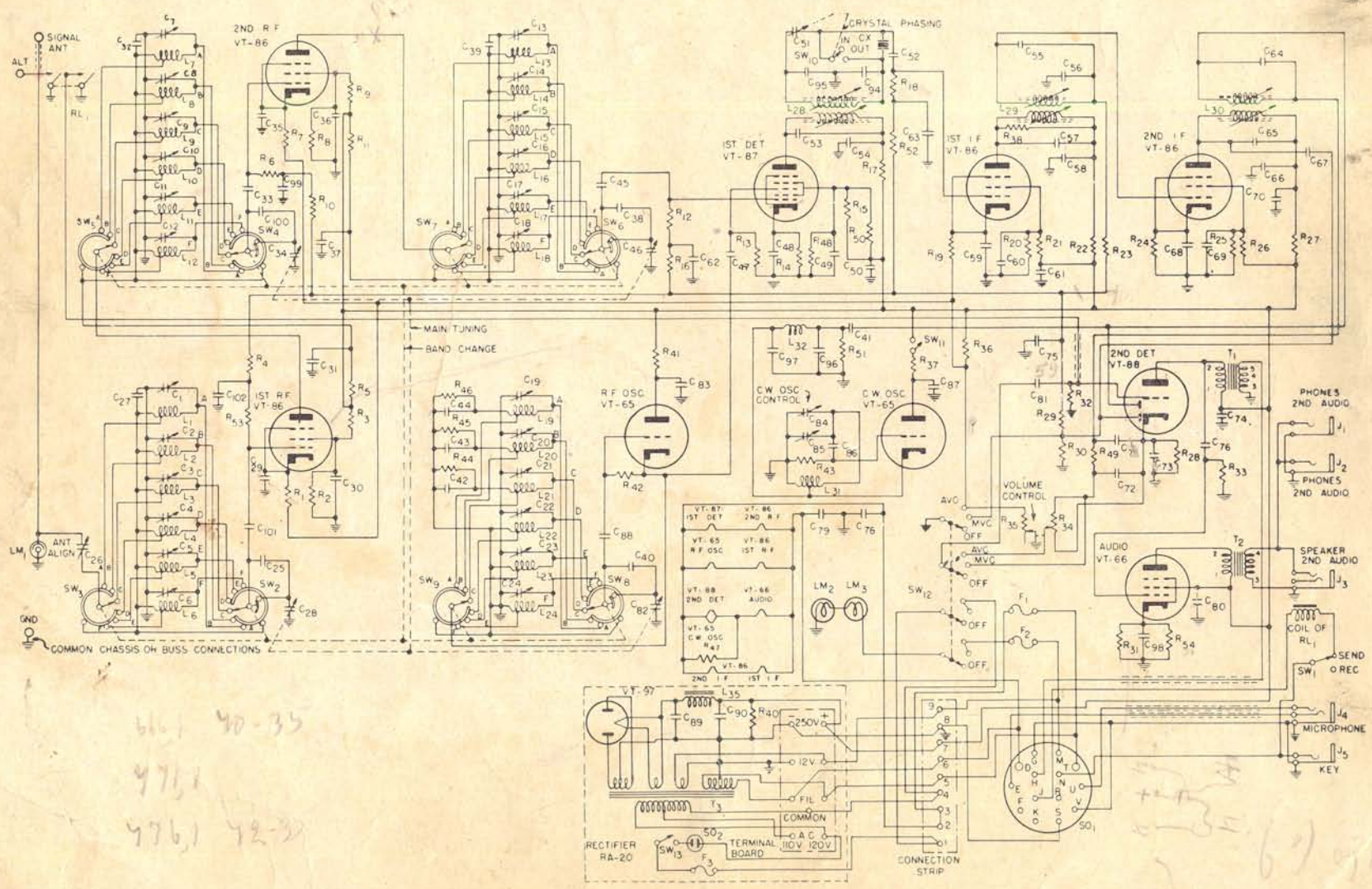
FIGURE 8, RADIO RECEIVER BC-342-N, CIRCUIT DIAGRAM.
