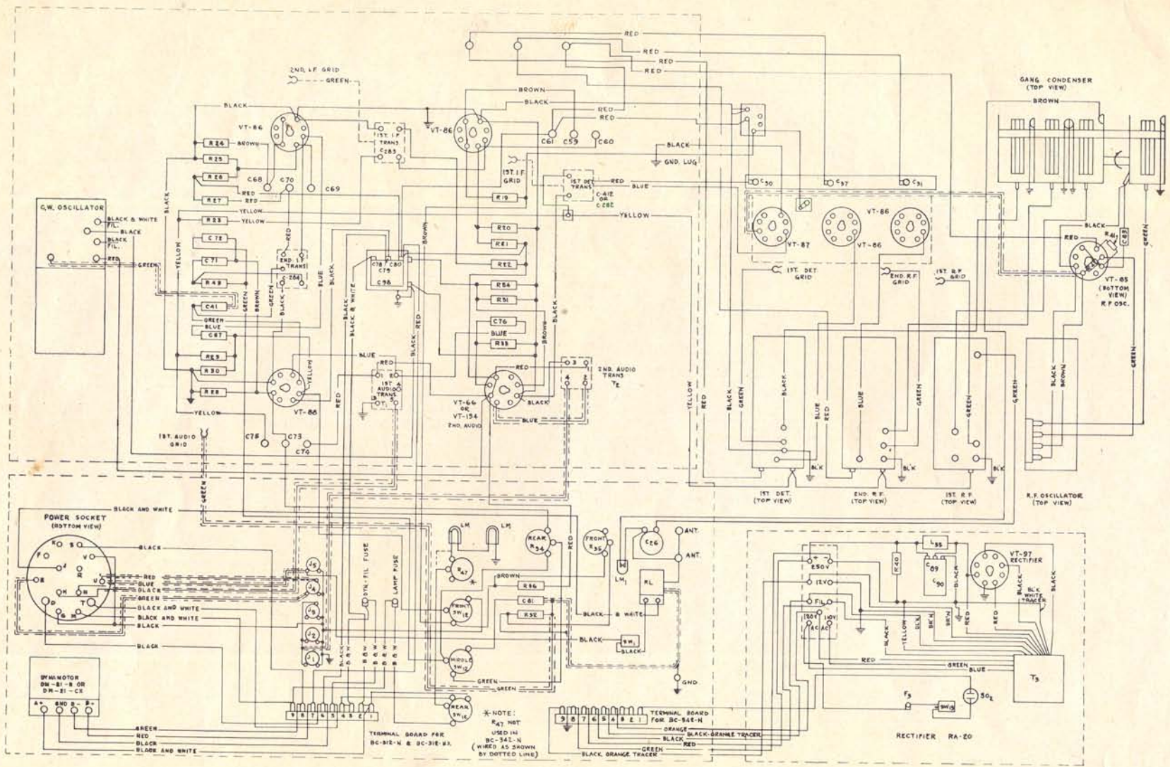
FIGURE 11. RADIO RECEIVERS BC-312-N, BC-312-NX AND BC-342-N, WIRING DIAGRAM.
