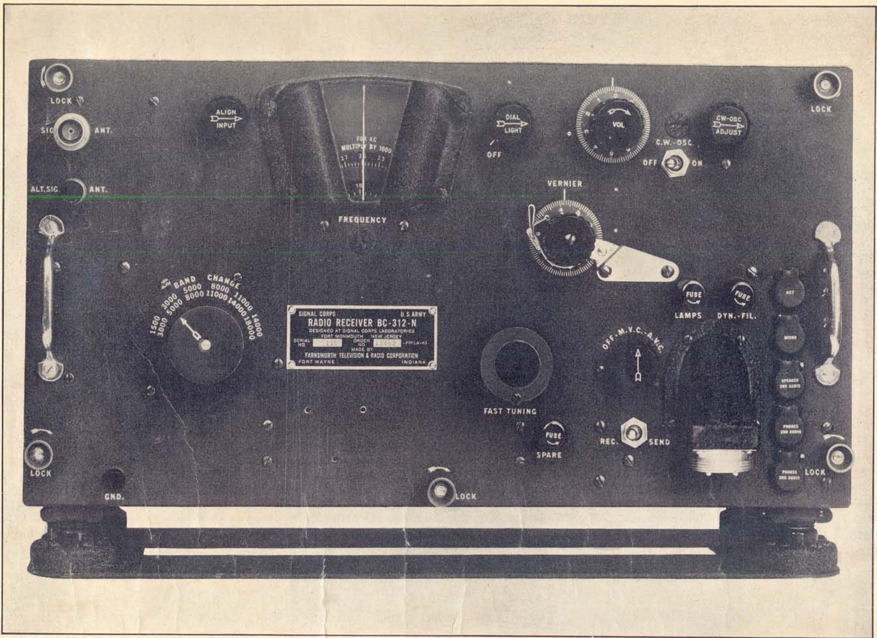
FIGURE 1. RADIO RECEIVER BC-312-N, FRONT VIEW.
