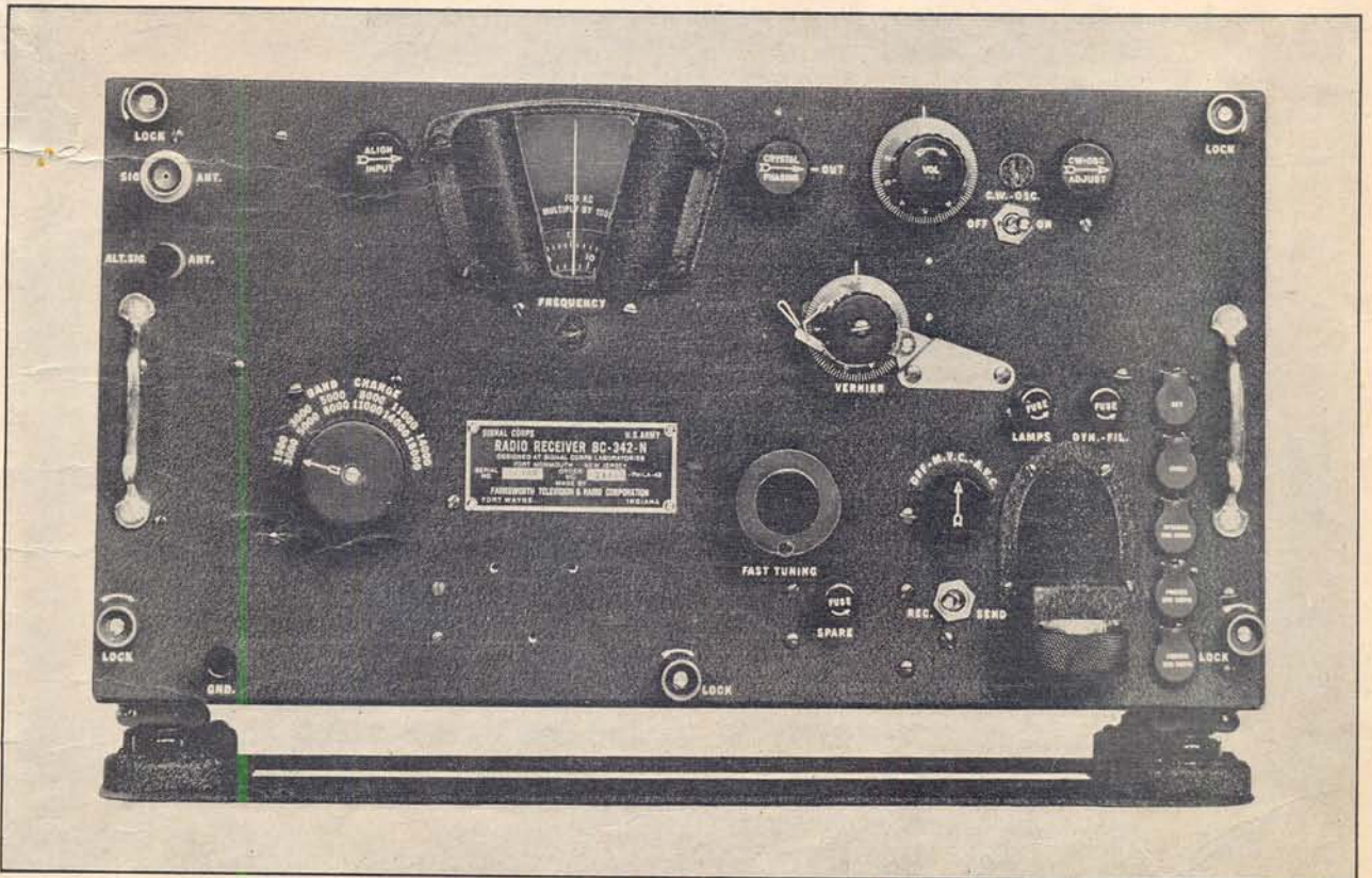
FIGURE 3, RADIO RECEIVER BC-342-N, FRONT VIEW.
