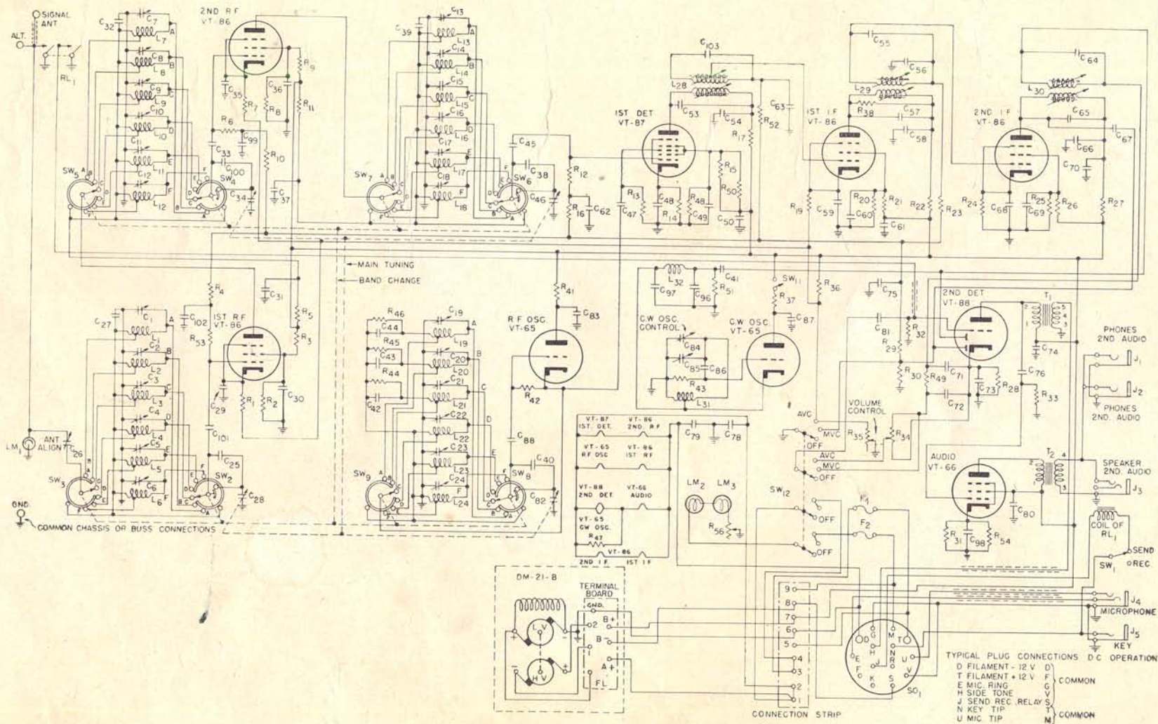
FIGURE 6, RADIO RECEIVER BC-312-N, CIRCUIT DIAGRAM.
