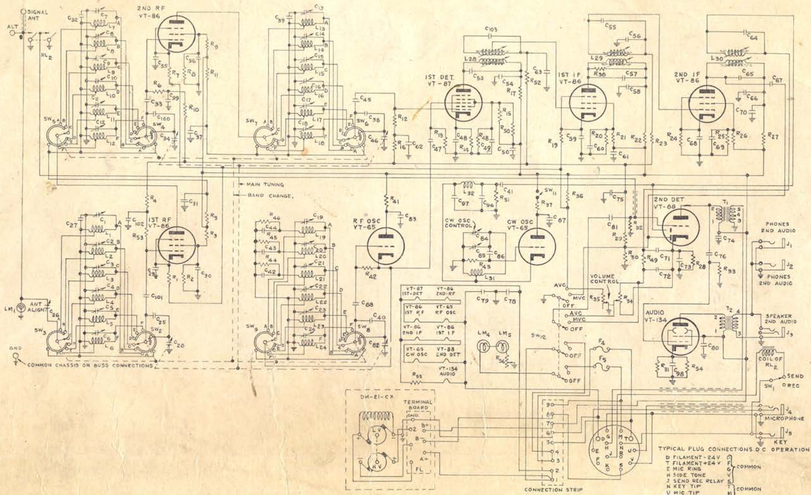
FIGURE 7, RADIO RECEIVER BC-312-NX, CIRCUIT DIAGRAM
