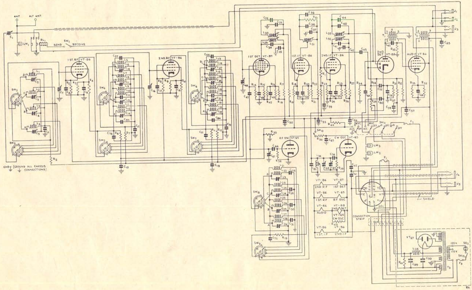
FIGURE 10, RADIO RECEIVER BC-344-D, CIRCUIT DIAGRAM.
