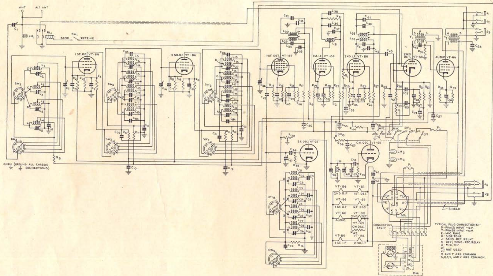
FIGURE 9, RADIO RECEIVER BC-314-G, CIRCUIT DIAGRAM.
