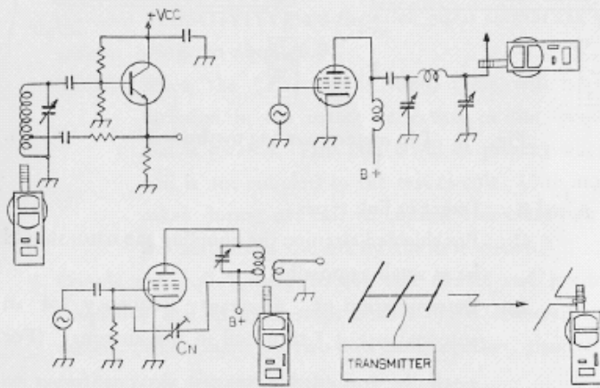
Fig. 2 Absorption wavemeter applications.
