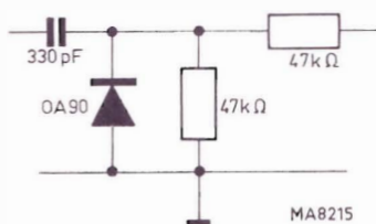
Fig. 22. Mixing circuit
