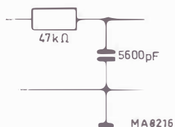
Fig. 23. Low-pass filter
