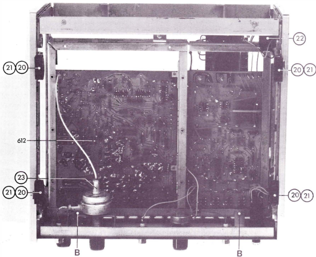
Fig. 34. Bottom view
