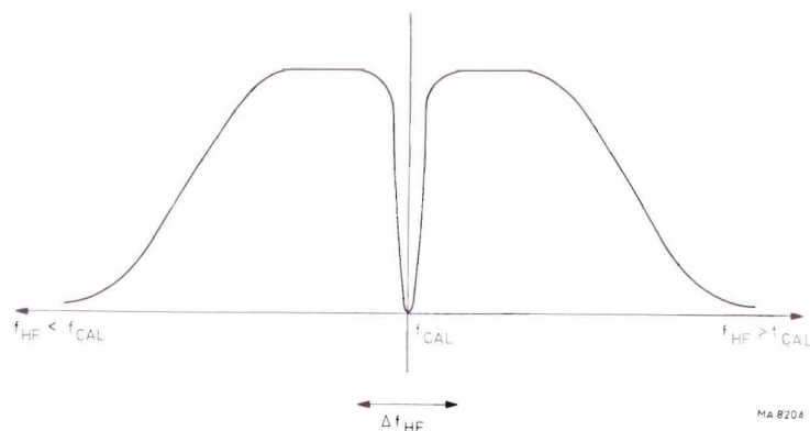
Fig. 28. Band-pass curve indicator
