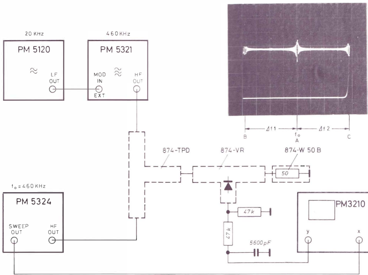
Fig. 31. Measuring set-up to determine the frequency sweep and the symmetry
