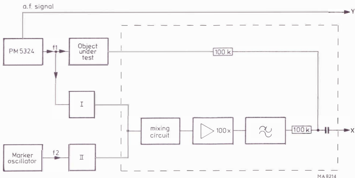
Fig. 21. Generating frequency markers
