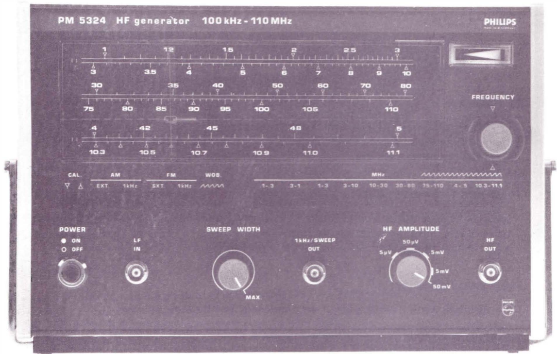
Fig. 4. Front view
