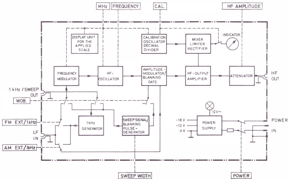
Fig. 2. Block diagram
