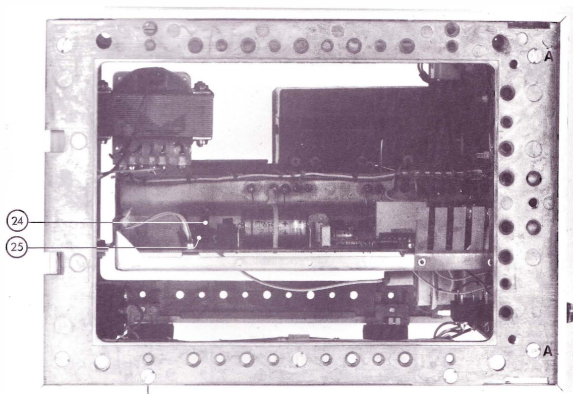
Fig. 36. Left-side view
