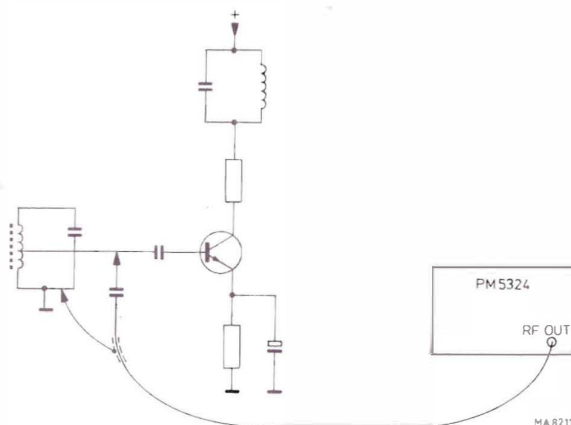
Fig. 11. Static adjustment of an AM receiver
