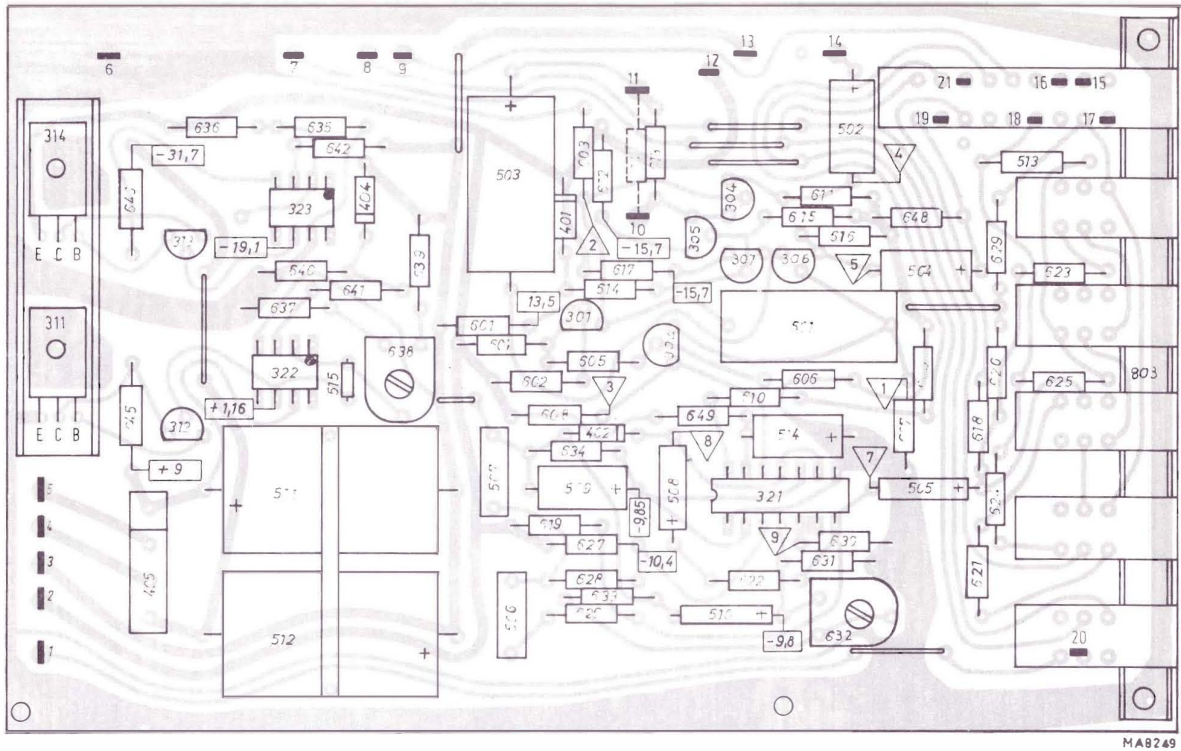
Fig. 41. Printed wiring board 2
