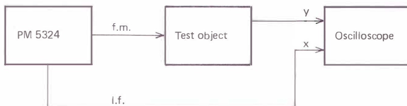
Fig. 7. Block diagram of the dynamic measuring method
